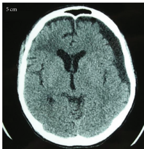
Figure 11-7. Subdural hematoma.
