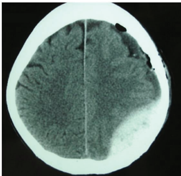
Figure 11-6. Epidural hematoma.
